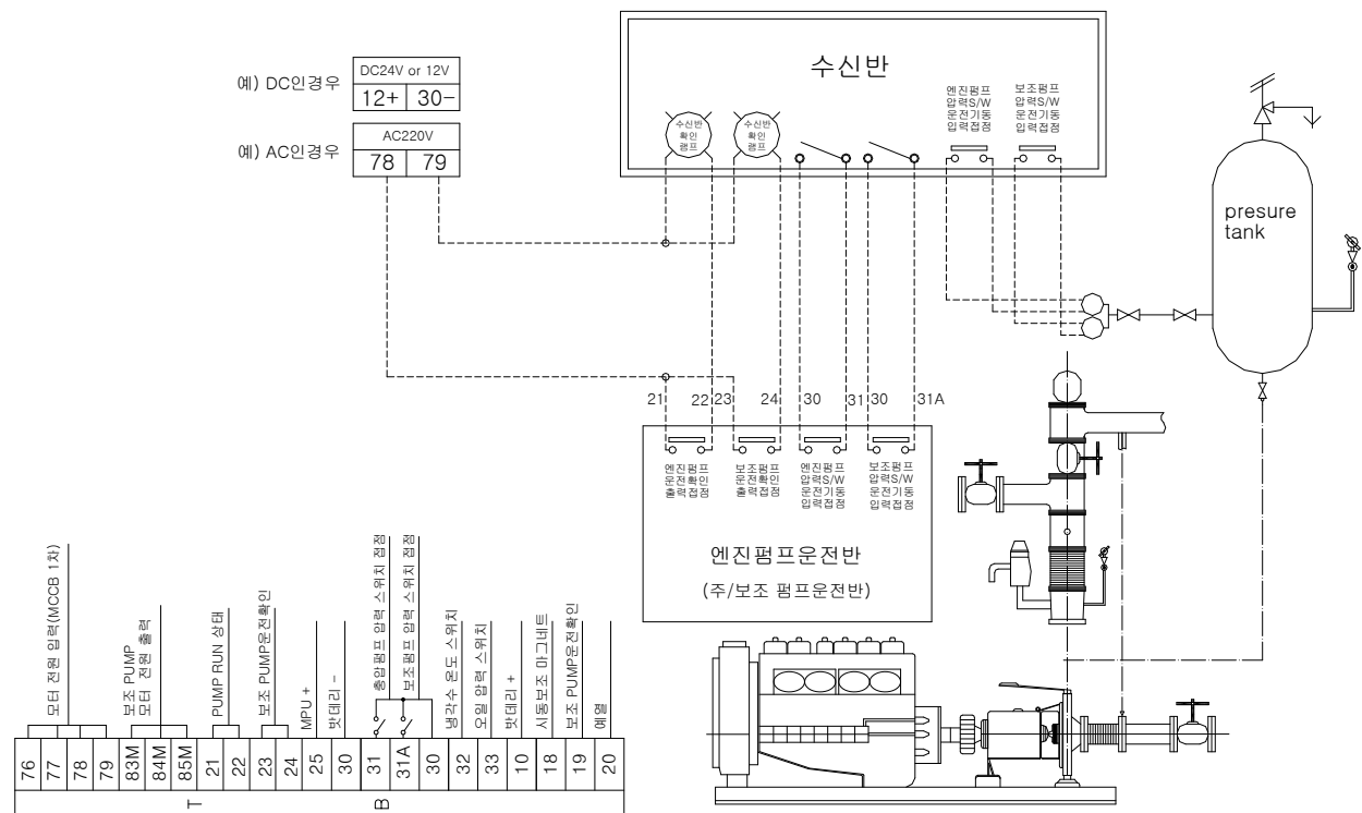
[회로도2]
