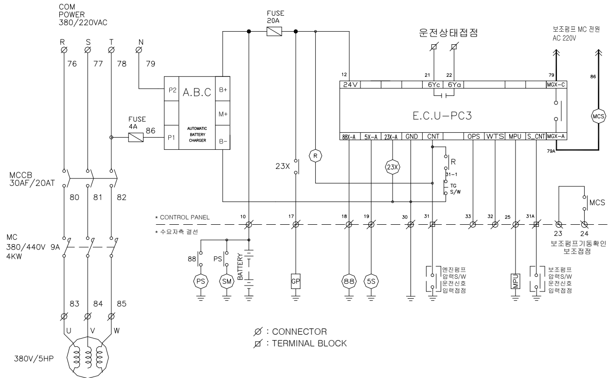
[회로도1]
